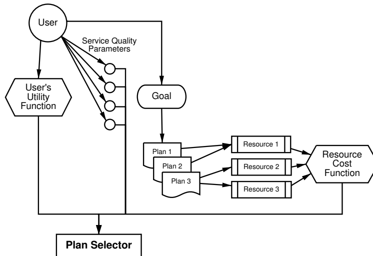
Figure 3: The plan selection mechanism
