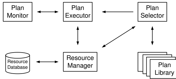
Figure 1: In our system, a plan selector chooses the best plan to achieve the user's goal from a plan library. The resource manager then assigns resources to this plan, using resources from its resource database. The resourced plan is then passed to the plan executor to be carried out. The plan monitor informs the plan executor as progress is made through the plan
